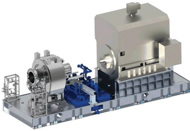
Figure 3. Elliott I40TCH Package And Maintenance Access
